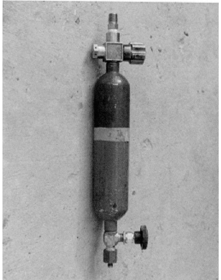
Typical 300cc sample cylinder used for butadiene.
